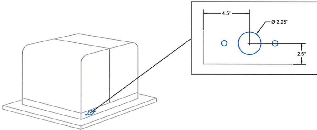
Figure # 5: Access Port for Temporary Service– Approximate Location
