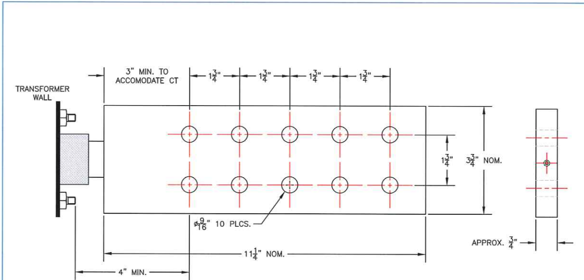
FIGURE #9 10-HOLE PAD FOR 1500 KVA AND ABOVE W/BUSHING SUPPORTS
