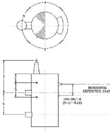
Figure # 1: Example of a Single Position Mounting
