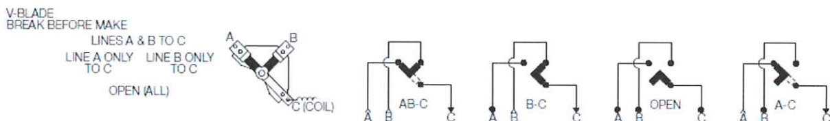
Figure # 6: Examples of a Primary Switch
