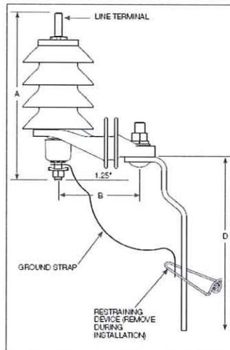
Figure # 2 - Example of Lightning Arrester to be installed on Transformer
