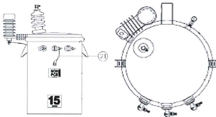
Figure # 3: Example of Mounted Lightning Arrester (Note: Item #21 is the transformer ground Strap)
