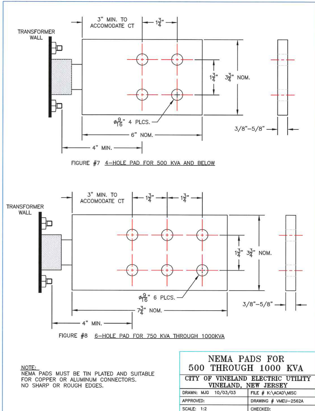
Figure # 8: Six-Hole Pad for 750kVA through 1000 kVA
